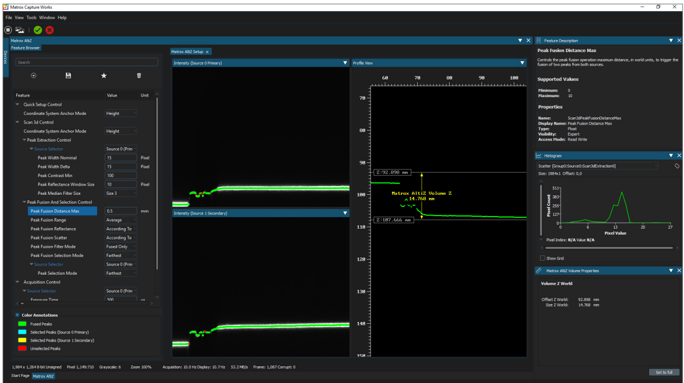
Peak (laser line) extraction, fusion, and volume (Z) adjustment within the Aurora Capture Works interactive utility.
